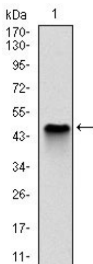
Figure 1: Western blot analysis using NQO1 mAb against human NQO1 (AA: 134-274) recombant protein. (Expected MW is 41.3 kDa)
